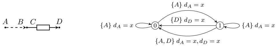
Fig. 3. LossyFIFO connector and its constraint automaton
